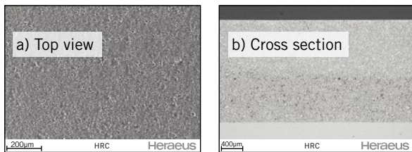
Figure 2 a) SEM micrograph of a typical HRC surface.
