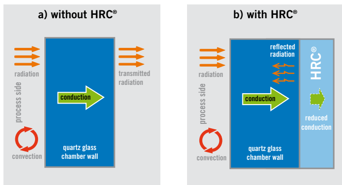
Figure 1: Illustration of the three heat transfer mechanisms.
