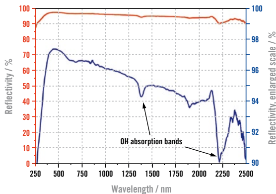
Figure 3: Reflection behavior of a typical HRC® surface.
