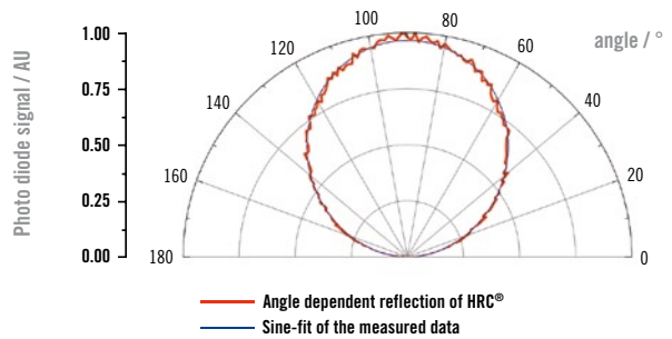
Figure 4: Typical directionality of the radiation reflected by HRC®.
